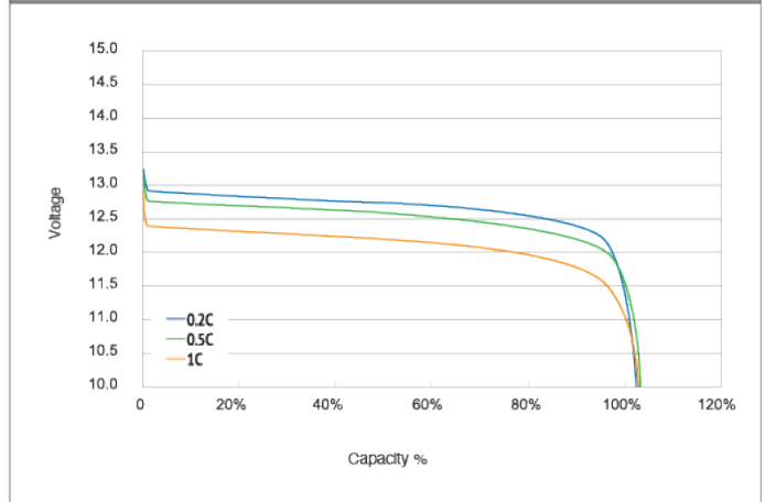
Discharging Characteristics (0.2C, 0.5C, 1C @25°C)
